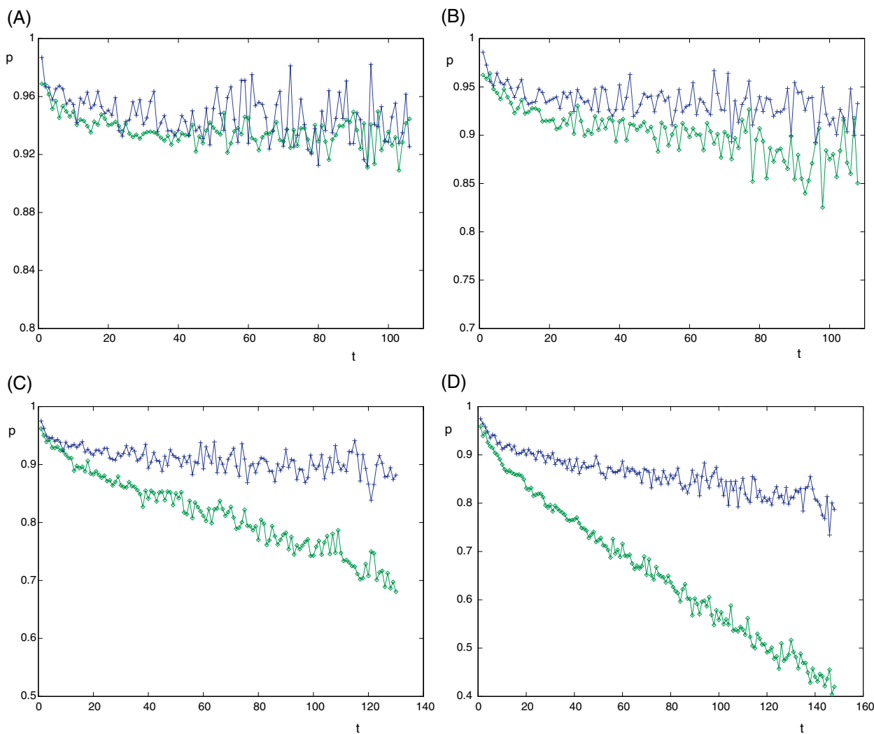
Fig. 5. Effects of the lattice topology on the reaction kinetics in a heterogeneous environment. We plot the index p versus time for reactions in a heterogeneous 2D plane with periodic boundary conditions. Here, P=0.2 and the initial conditions are A_0=0.01 , B_0=0.1 . The plots are generated by averaging over 500 samples of data obtained from a 500 \times 500 square lattice LGA (green data points) and a 500 \times 500 triangular lattice LGA (blue data points). Molecules of all species ( A , B and C ) are mobile. The static obstacle concentration is (A) [O]=0.1 , (B) [O]=0.2 , (C) [O]=0.3 , (D) [O]=0.4 .
